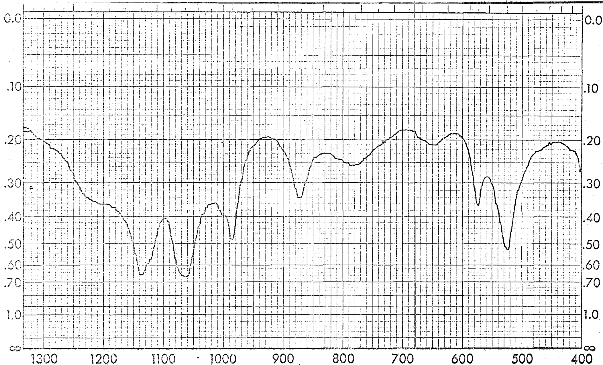
Spectrum No. 17: 50% Magnesium Ammonium Phosphate, MgNH_4PO_4 , and 50% Calcium Hydrogen Phosphate, CaHPO_4 By Transmission I.R.
