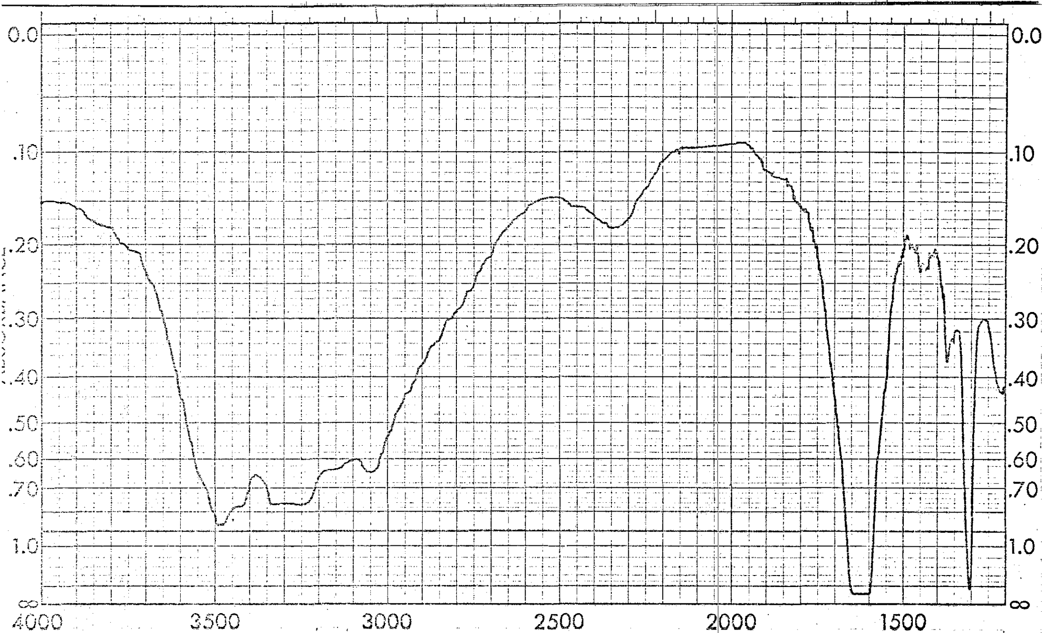
Spectrum No. 52: 25% Magnesium Phosphate, MgHPO_4 , 25% Calcium Hydrogen Phosphate, CaHPO_4 , 25% Magnesium Ammonium Phosphate, MgNH_4PO_4 , and 25% Calcium Oxalate Monohydrate, CaC_2O_4 \cdot H_2O By Transmission I.R.
