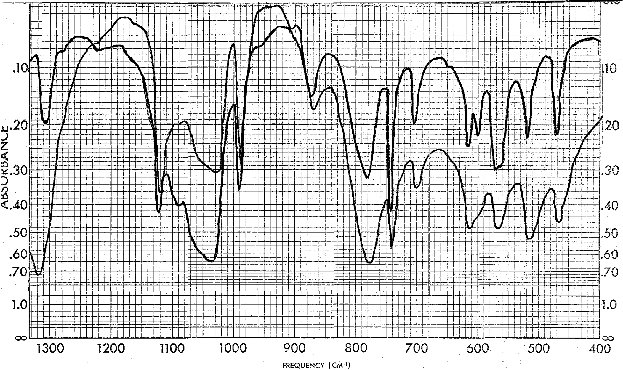
Figure 8. Spectrum of 50% uric acid, C_5H_4N_4O_3 and 50% tricalcium phosphate, Ca_3(PO_4)_2 (red) and a urinary calculus (blue) by transmission I.R.
