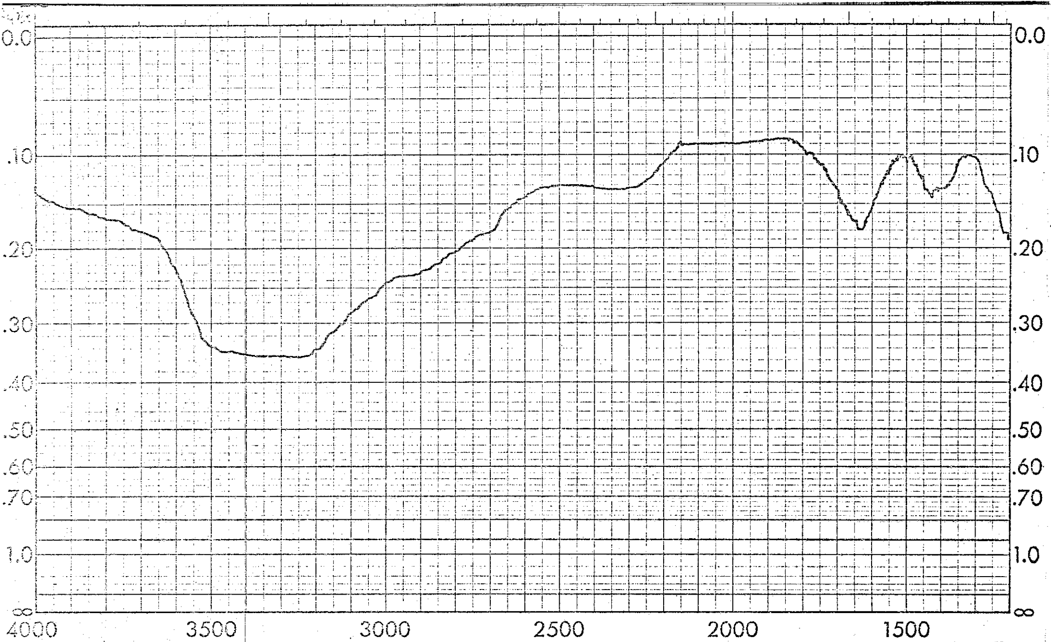
Spectrum No. 44: 50% Magnesium Ammonium Phosphate, MgNH_4PO_4 , 25% Magnesium Phosphate, MgHPO_4 , and 25% Tricalcium Phosphate, Ca_3(PO_4)_2 By Transmission I.R.
