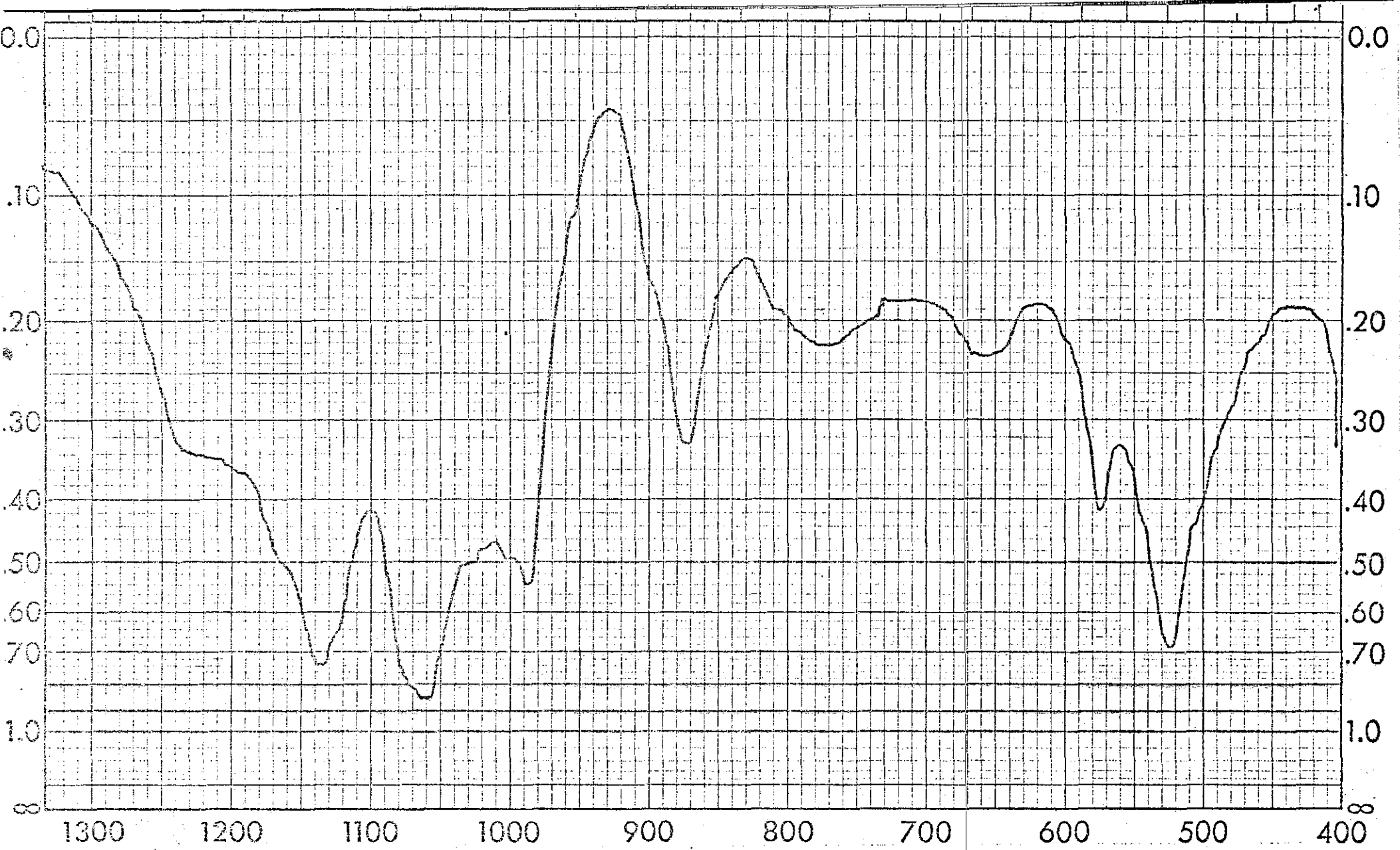
Spectrum No. 11: 50% Magnesium Phosphate, MgHPO_4 , and 50% Calcium Hydrogen Phosphate, CaHPO_4 By Transmission I.R.
