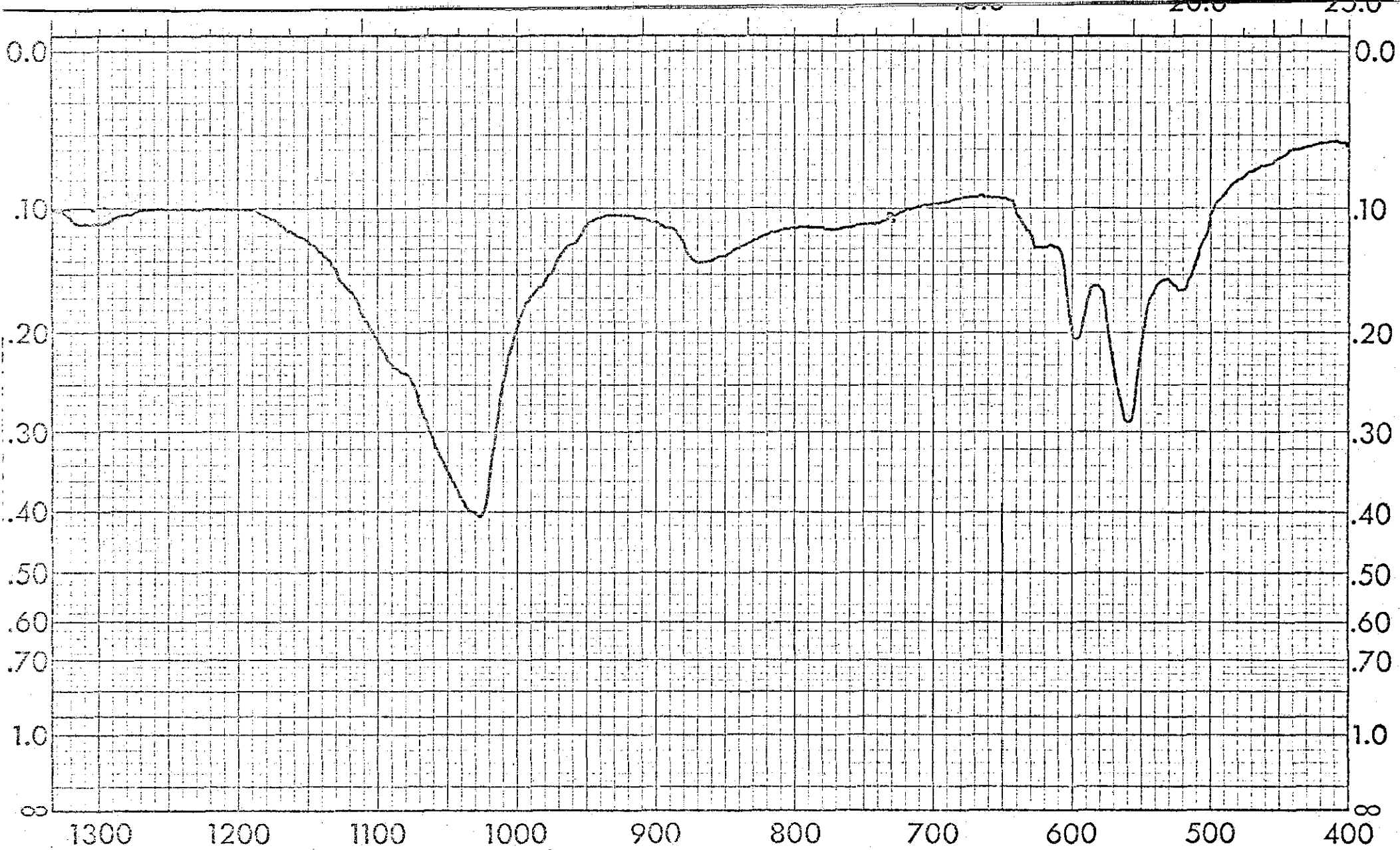
Spectrum No. 94: 50% Tricalcium Phosphate, \text{Ca}_3(\text{PO}_4)_2 , 25% Calcium Hydrogen Phosphate, \text{CaHPO}_4 , and 25% Magnesium Phosphate, \text{MgHPO}_4 by A.T.R.
