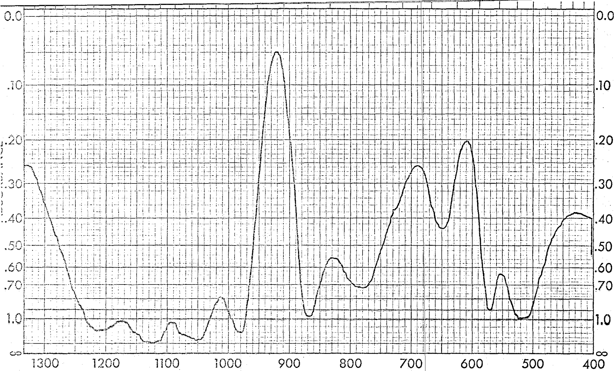
Spectrum No. 3: Calcium Hydrogen Phosphate, CaHPO 4 By Transmission I.R.
