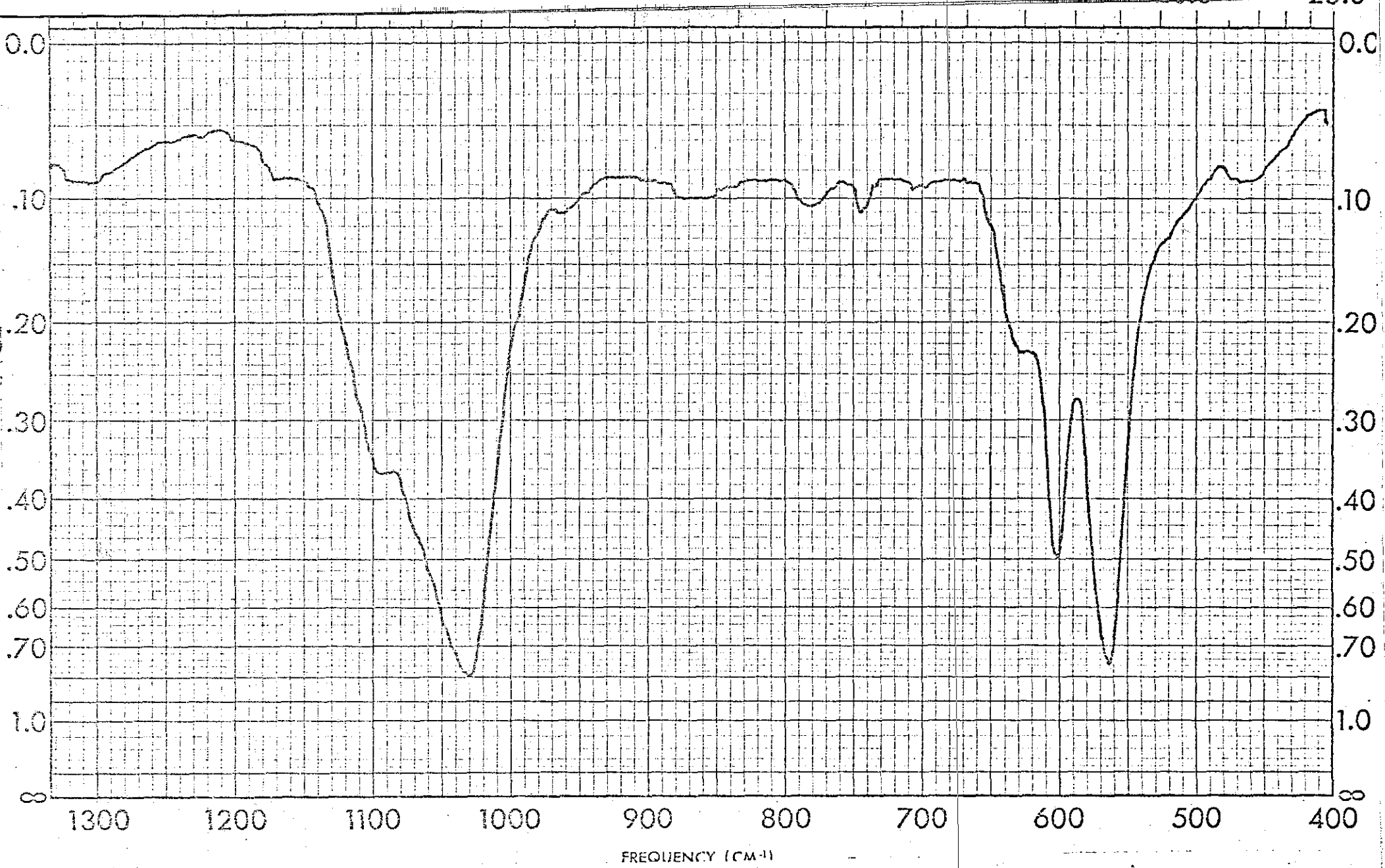
Spectrum No. 64: Tricalcium Phosphate, \text{Ca}_3(\text{PO}_4)_2 by A.T.R.
