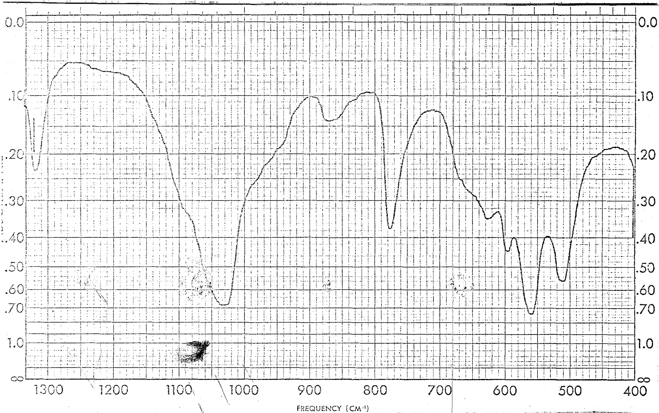
Spectrum No. 111: 25% Magnesium Ammonium Phosphate, \text{MgNH}_4\text{PO}_4 , 25% Calcium Hydrogen Phosphate, \text{CaHPO}_4 , 25% Tricalcium Phosphate, \text{Ca}_3(\text{PO}_4)_2 , and 25% Calcium Oxalate Monohydrate,
