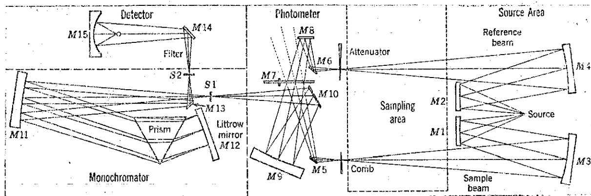
Figure 5. Optical system of double-beam infrared spectrophotometer. (28)
