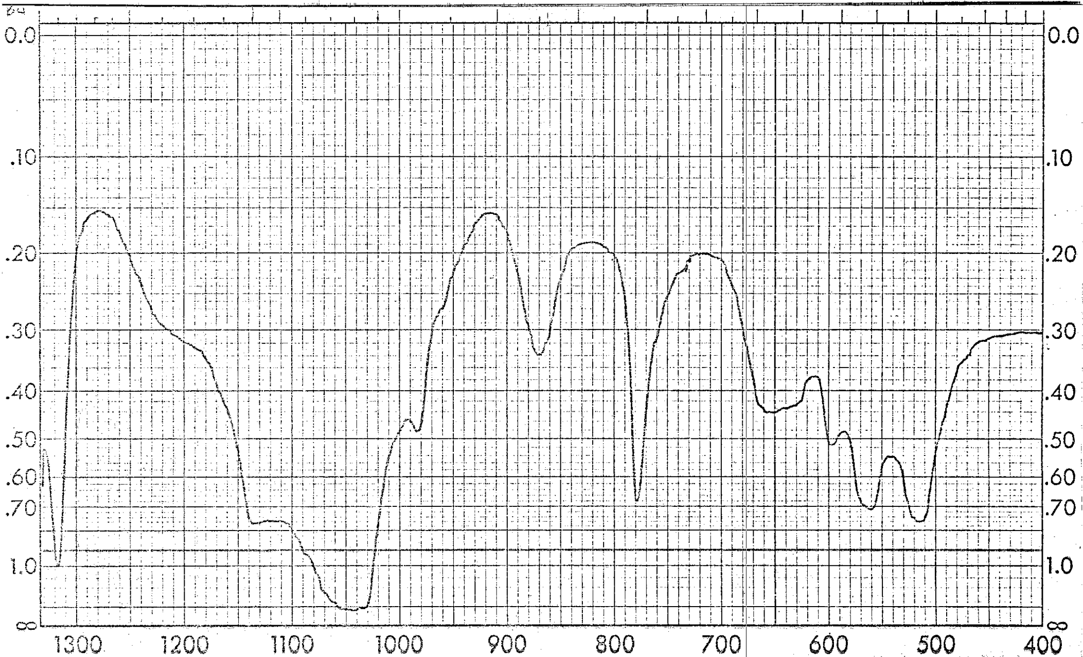
Spectrum No. 54: 25% Magnesium Ammonium Phosphate, MgNH_4PO_4 , 25% Calcium Hydrogen Phosphate, CaHPO_4 , 25% Tricalcium Phosphate, Ca_3(PO_4)_2 , and 25% Calcium Oxalate Monohydrate,
