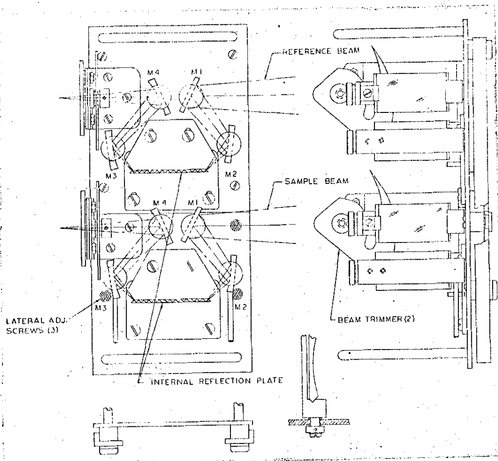
Figure 6. Working Diagram of Model 12 Wilks Scientific Corporation Double Beam Attachment(30)
