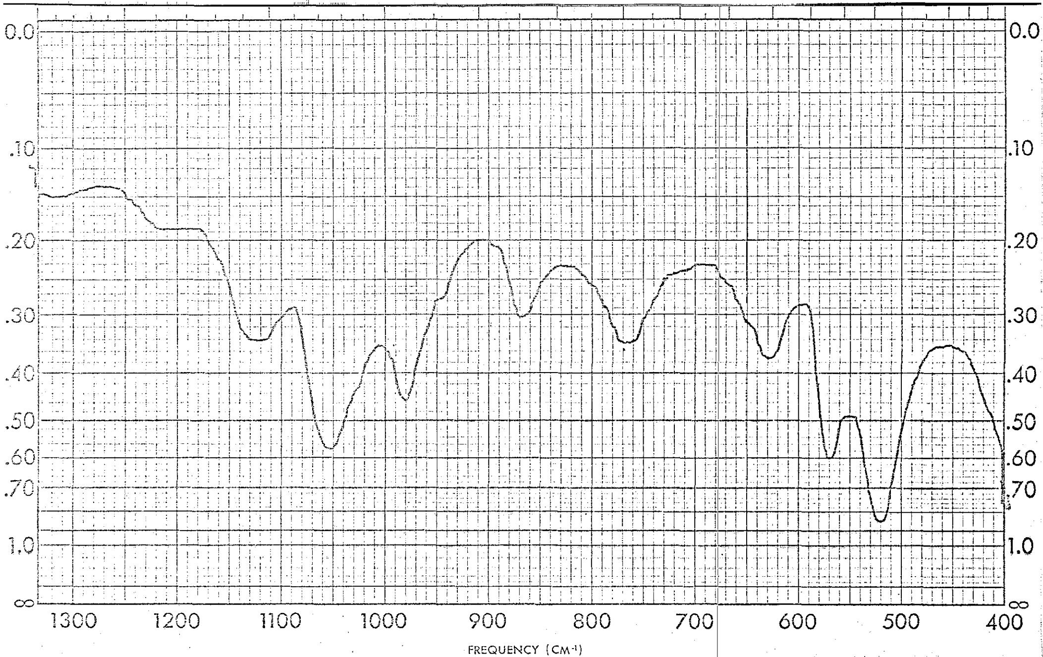
Spectrum No. 109: 50% Calcium Hydrogen Phosphate, \text{CaHPO}_4 , 25% Magnesium Phosphate, \text{MgHPO}_4 , and 25% Magnesium Ammonium Phosphate,
