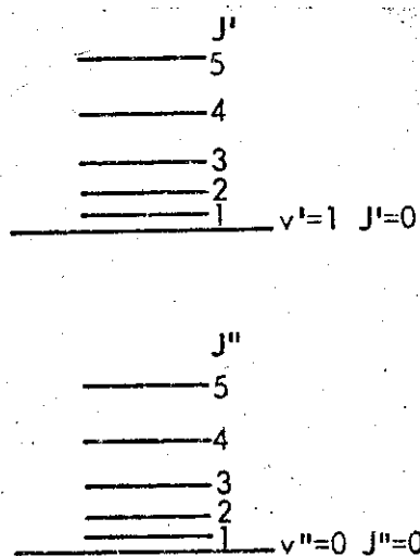
Figure 1. A vibrational-rotational energy level diagram.
