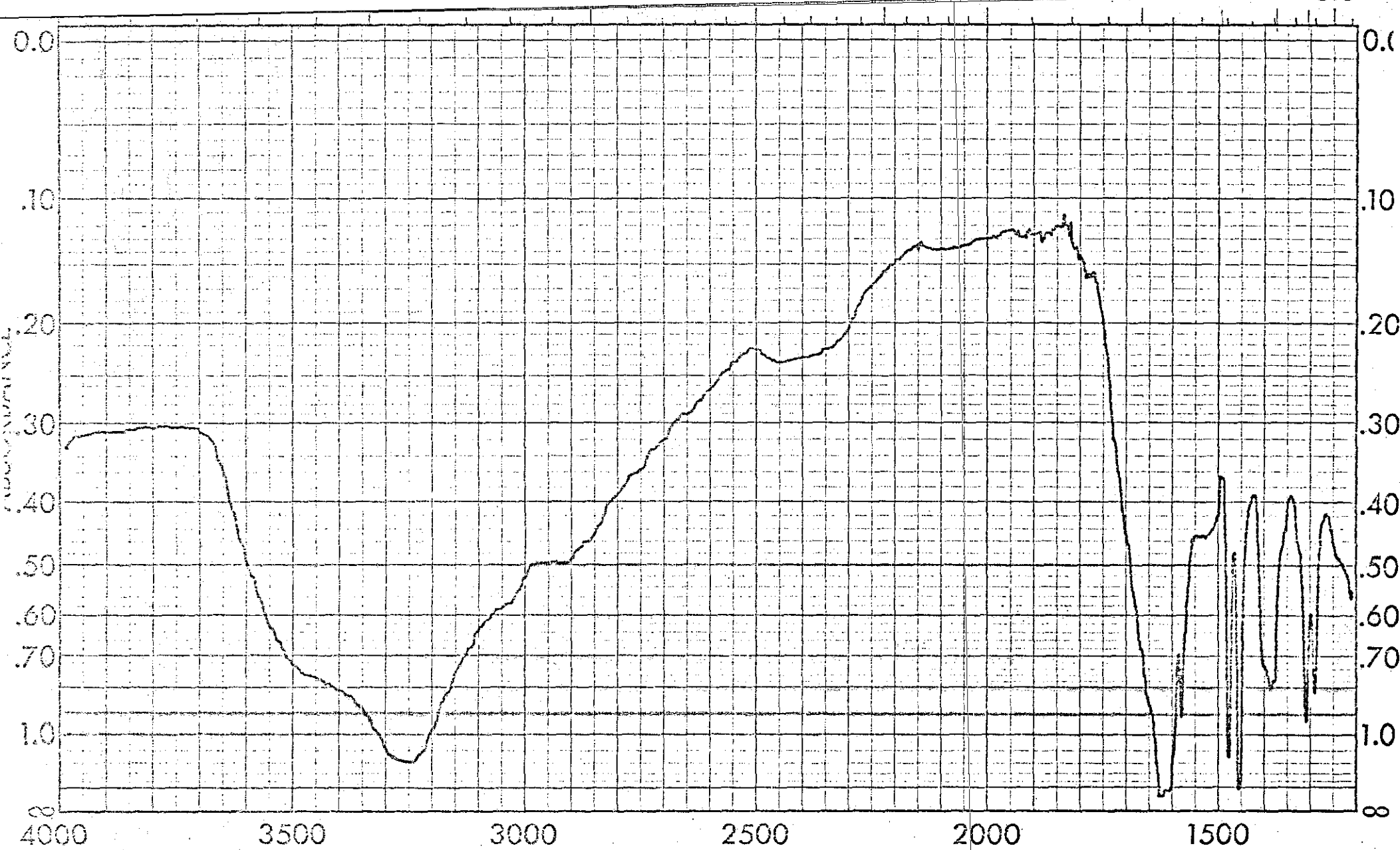
Spectrum No. 15: 50% Indigo, C_{16}H_{10}N_2O_2 , and 50% Magnesium Phosphate, MgHPO_4 By Transmission. I.R.
