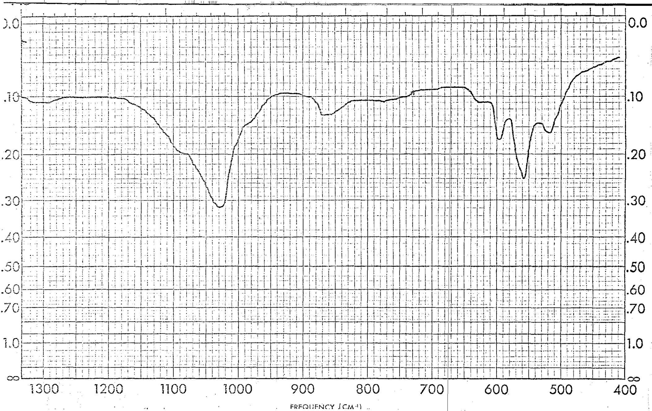
Spectrum No. 78: 50% Magnesium Phosphate, MgHPO_4 , and 50% Calcium Hydrogen Phosphate, CaHPO_4 by A.T.R.
