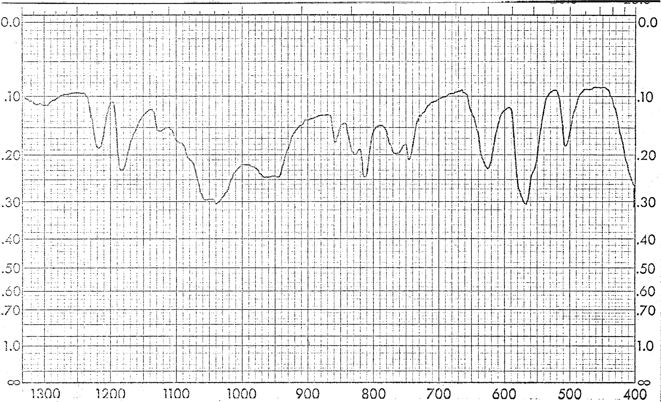
Spectrum No. 88: 50% Cystine, \text{SCH}_2\text{CH}(\text{NH}_2)\text{-COOH} , and 50% Magnesium Ammonium Phosphate, \text{MgNH}_4\text{PO}_4 by A.T.R.
