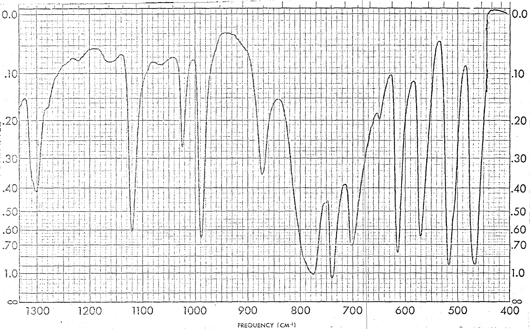
Spectrum No. 62: Uric Acid, \text{C}_5\text{H}_4\text{N}_4\text{O}_3 by A.T.R.
