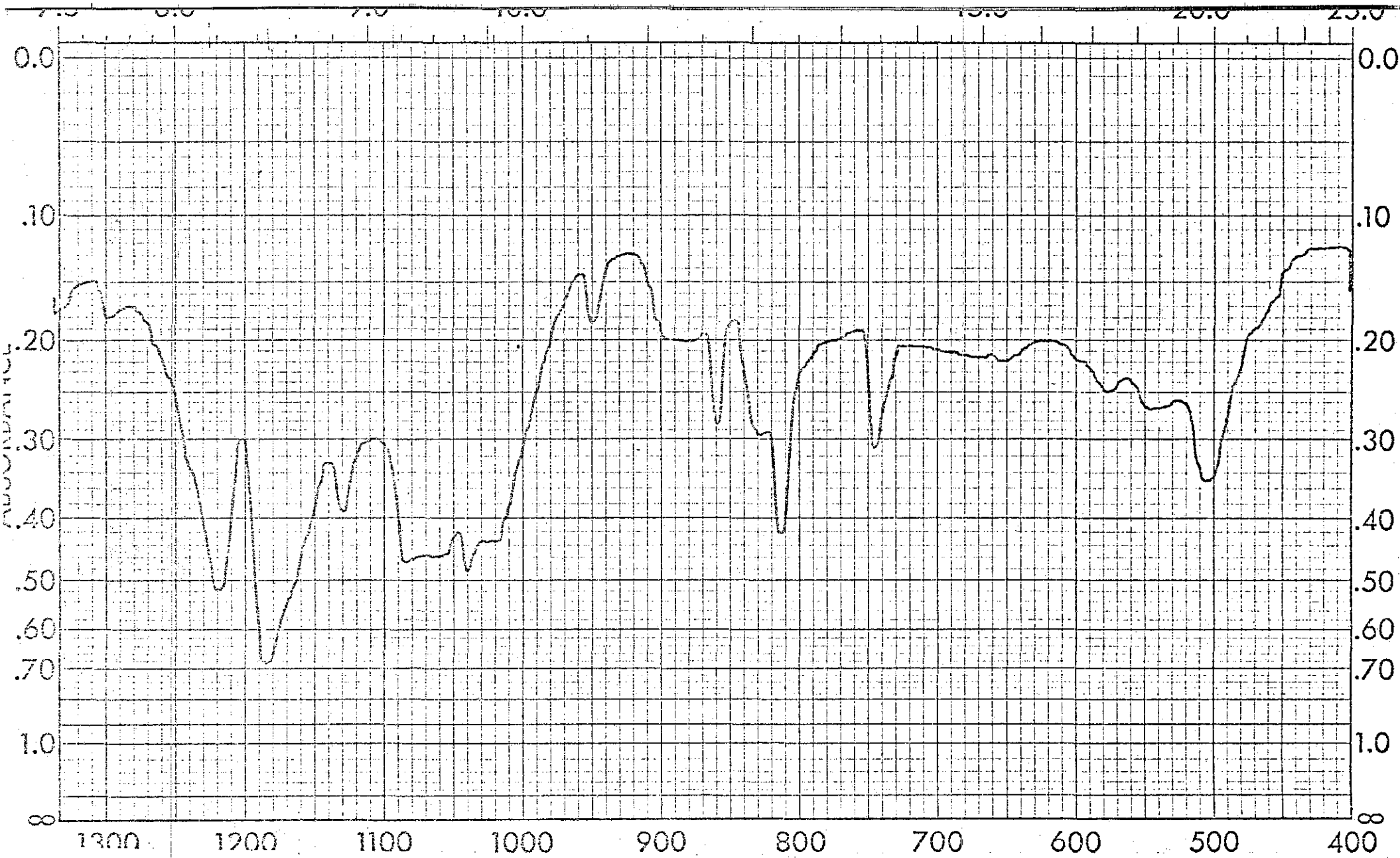
Spectrum No. 34: 50% Magnesium Phosphate, MgHPO_4 , and 50% Cystine, SCH_2CH(NH_2)-COOH By Transmission I.R.
