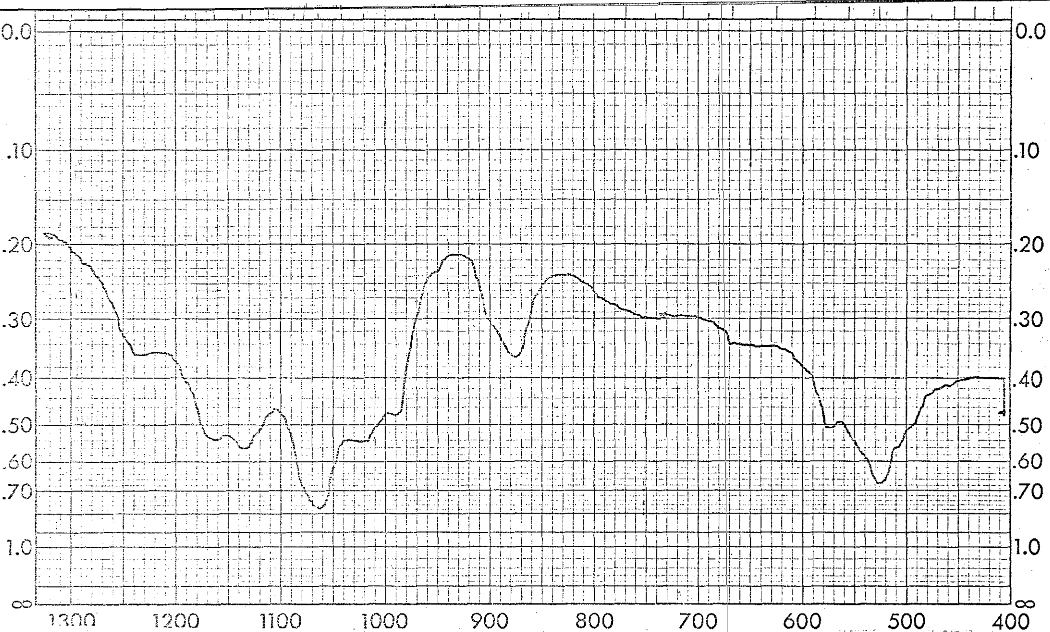
Spectrum No. 51: 50% Magnesium Phosphate, MgHPO_4 , 25% Magnesium Ammonium Phosphate, MgNH_4PO_4 , and 25% Calcium Hydrogen Phosphate, CaHPO_4 By Transmission I.R.
