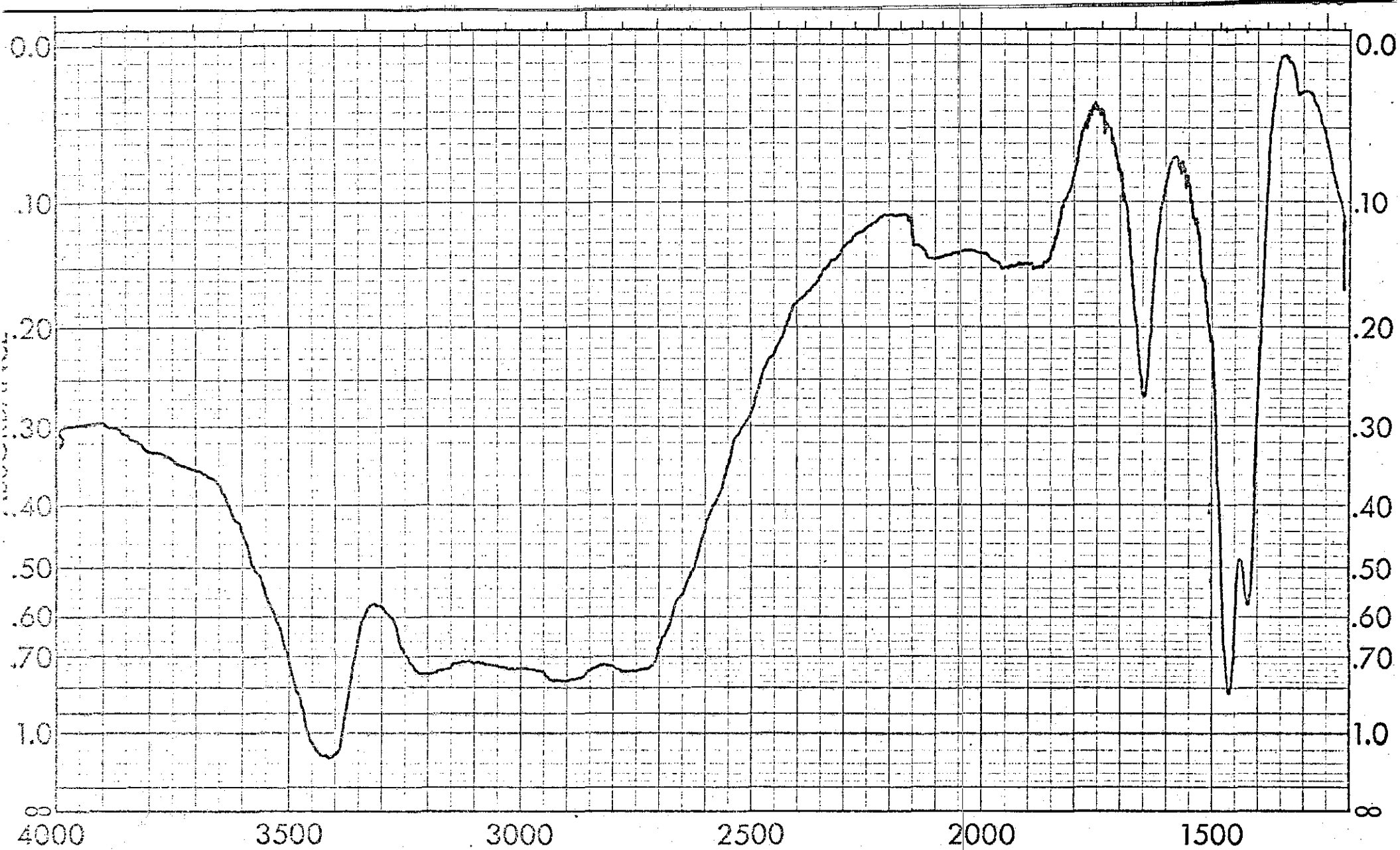
Spectrum No. 4: Magnesium Ammonium Phosphate Hexahydrate,
