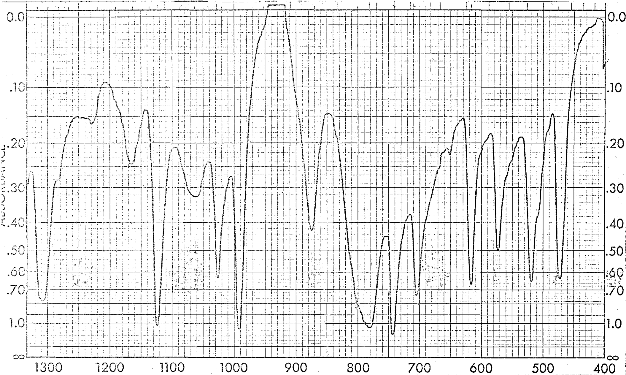
Spectrum No. 25: 50% Magnesium Phosphate, MgHPO_4 , and 50% Uric Acid, C_5H_4N_4O_3 By Transmission I.R.
