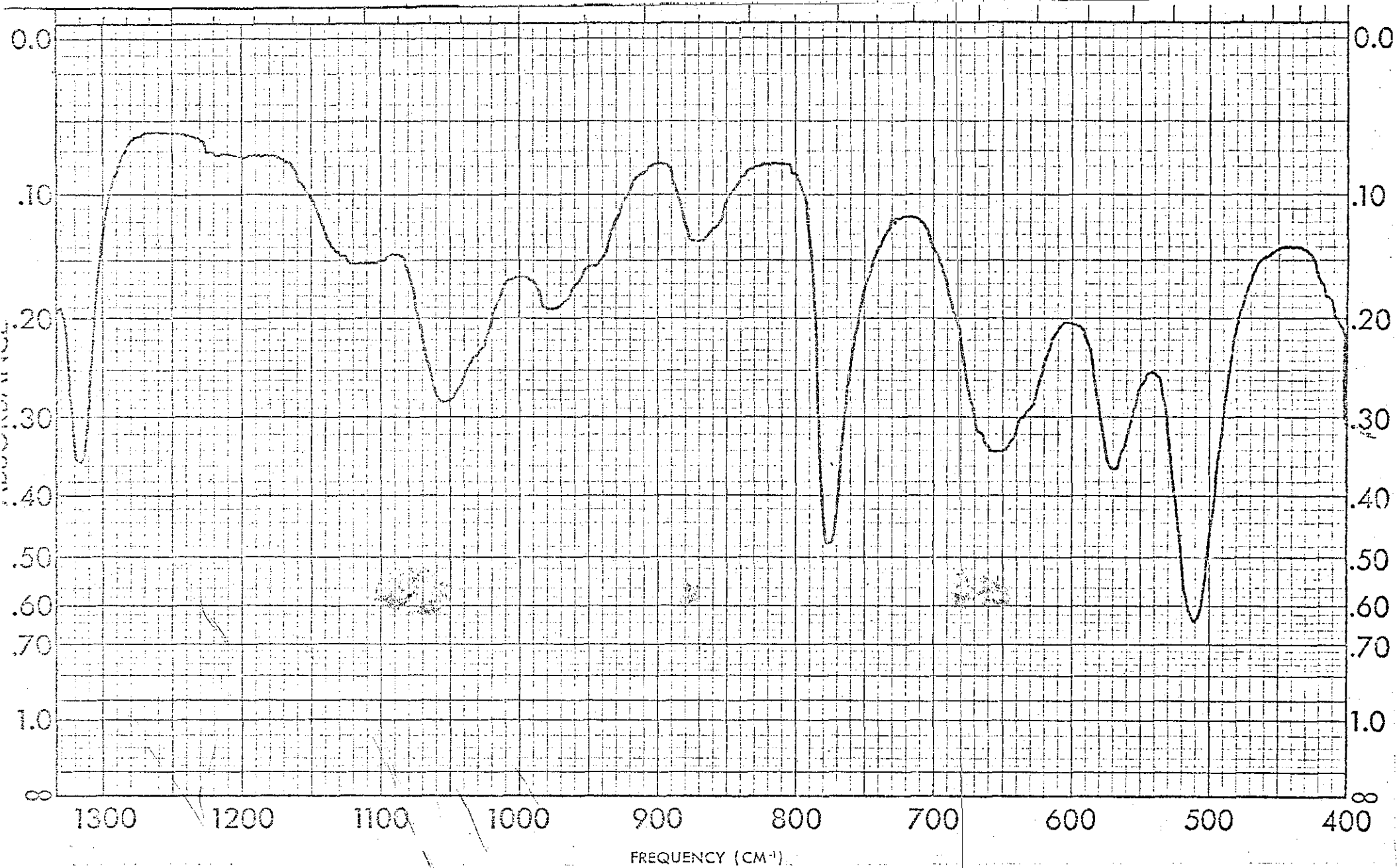
Spectrum No. 106: 50% Calcium Oxalate Monohydrate, \text{CaC}_2\text{O}_4 \cdot \text{H}_2\text{O} , 25% Calcium Hydrogen Phosphate, \text{CaHPO}_4 , and 25% Magnesium Ammonium
