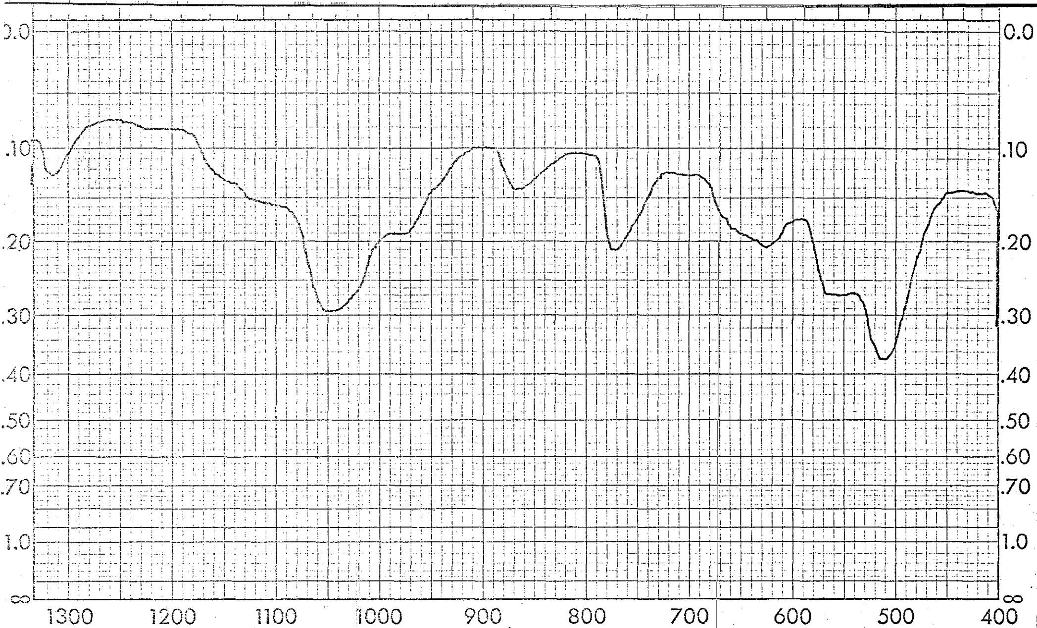
Spectrum No. 104: 25% Calcium Oxalate Monohydrate, \text{CaC}_2\text{O}_4 \cdot \text{H}_2\text{O} , 25% Calcium Hydrogen Phosphate, \text{CaHPO}_4 , 25% Magnesium Ammonium Phosphate, \text{MgNH}_4\text{PO}_4 , and 25% Magnesium
