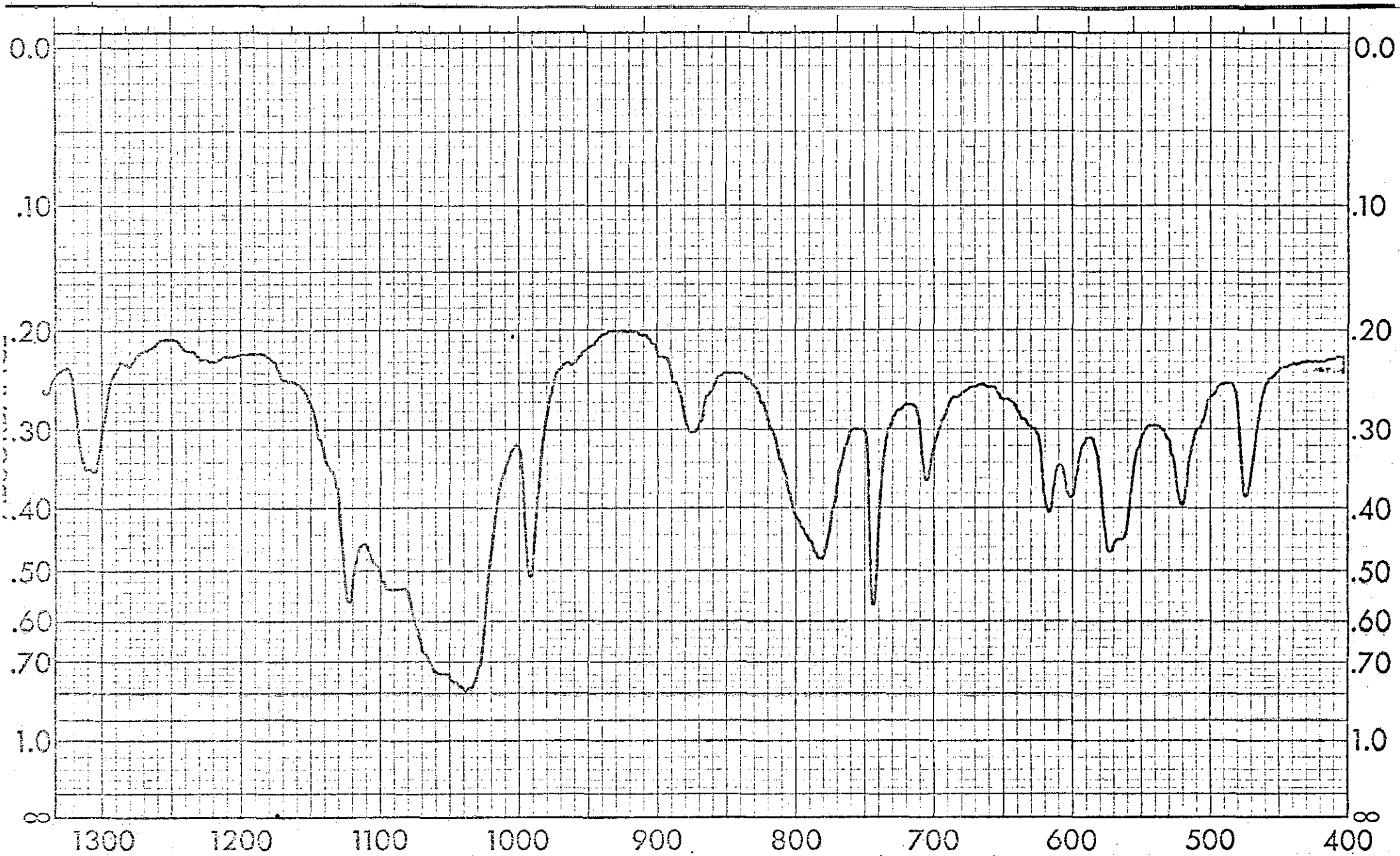
Spectrum No. 27: 50% Uric Acid, C_5H_4N_4O_3 , and 50% Tricalcium Phosphate, Ca_3(PO_4)_2 By Transmission I.R.
