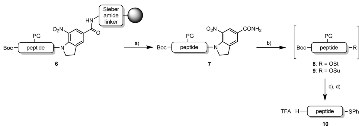
Scheme 2. Photochemical synthesis of peptide- \alpha -phenylthioesters via a peptide-OBt or OSu ester intermediate (not isolated). a) 1% TFA in CH 2 Cl 2 ; b) hν (350 nm), argon, THF or DMF, HOBt or HOSu; c) PhSH; d) TFA/H 2 O/TIS (95:2.5:2.5). TIS = triisopropylsilane.
